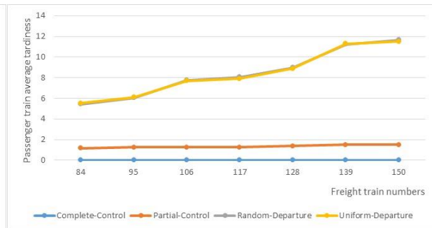
Figure 2. Passenger Train Average Tardiness (min)
